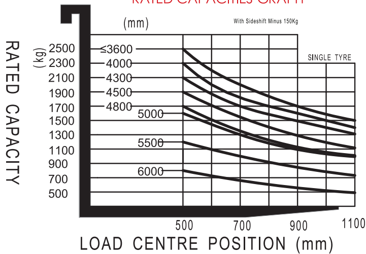
CPD25F8 RATED CAPACITIES GRAPH
