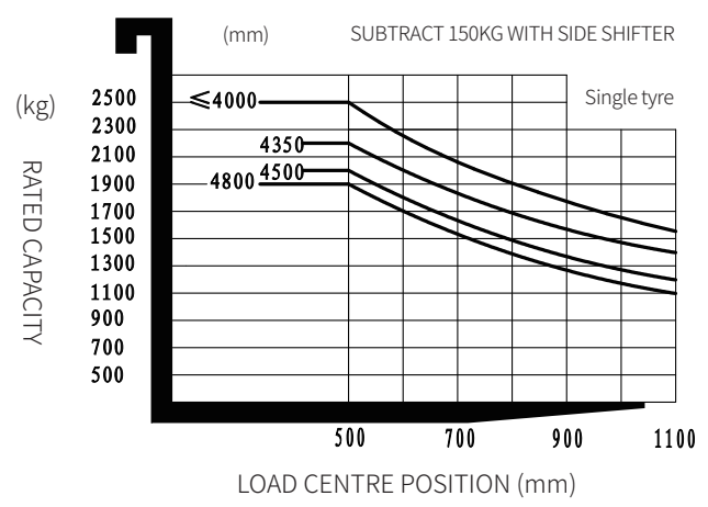
RATED CAPACITIES AND LOAD CENTERS GRAPH
